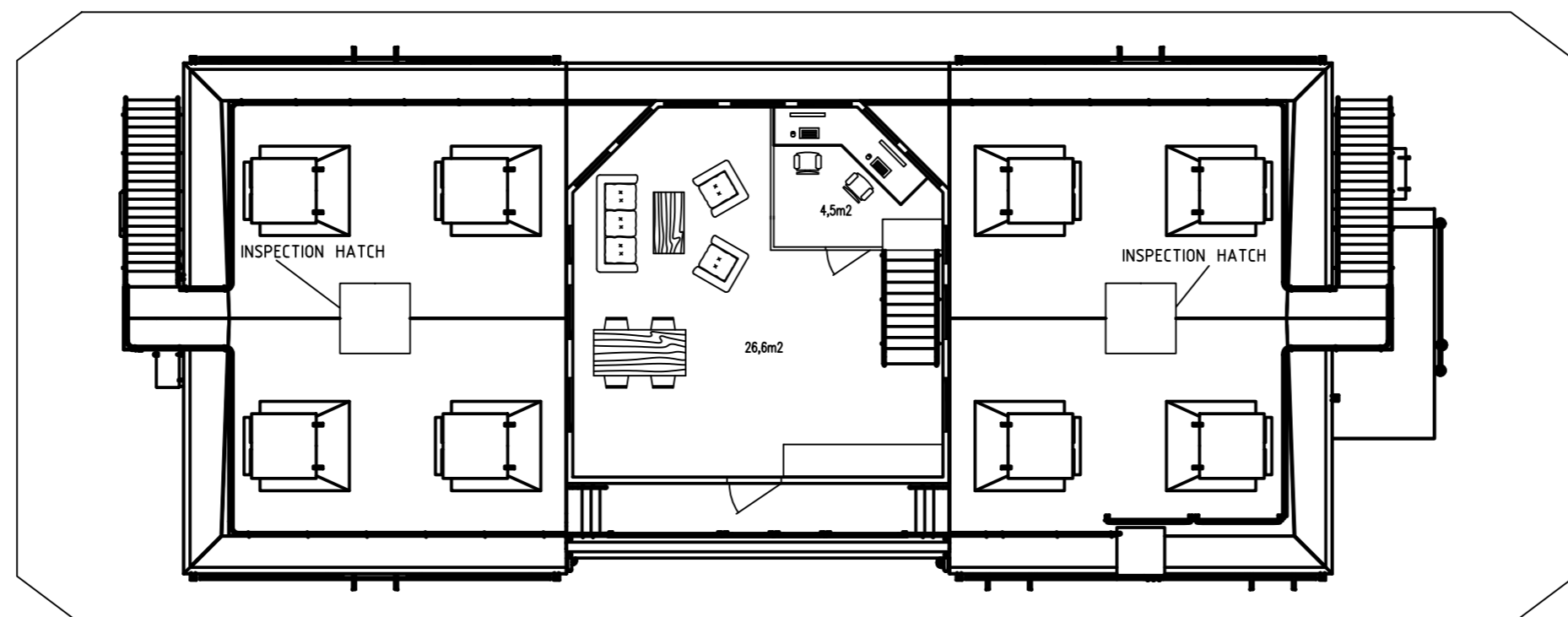
SILO DECK TOTAL ACCOMMODATION SPACE 31,8 m 2
